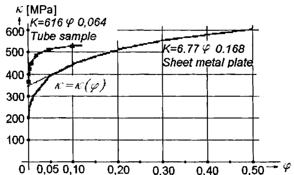
Fig. 3. Flow curve of RSt.37-2
