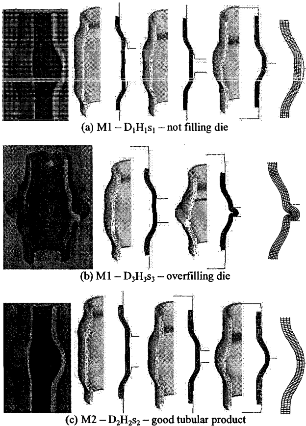
Fig. 5. Physical and numerical models of tubular specimens
