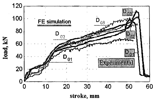
Fig. 6. Comparative load-stroke diagrams, H_2=69\text{mm} , s_2=2.33\text{mm}
